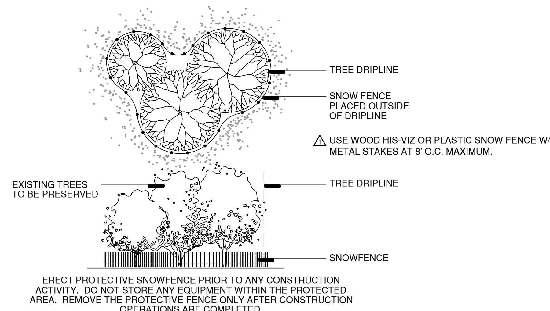
1 A Typical Tree Preservation Fencing NTS
