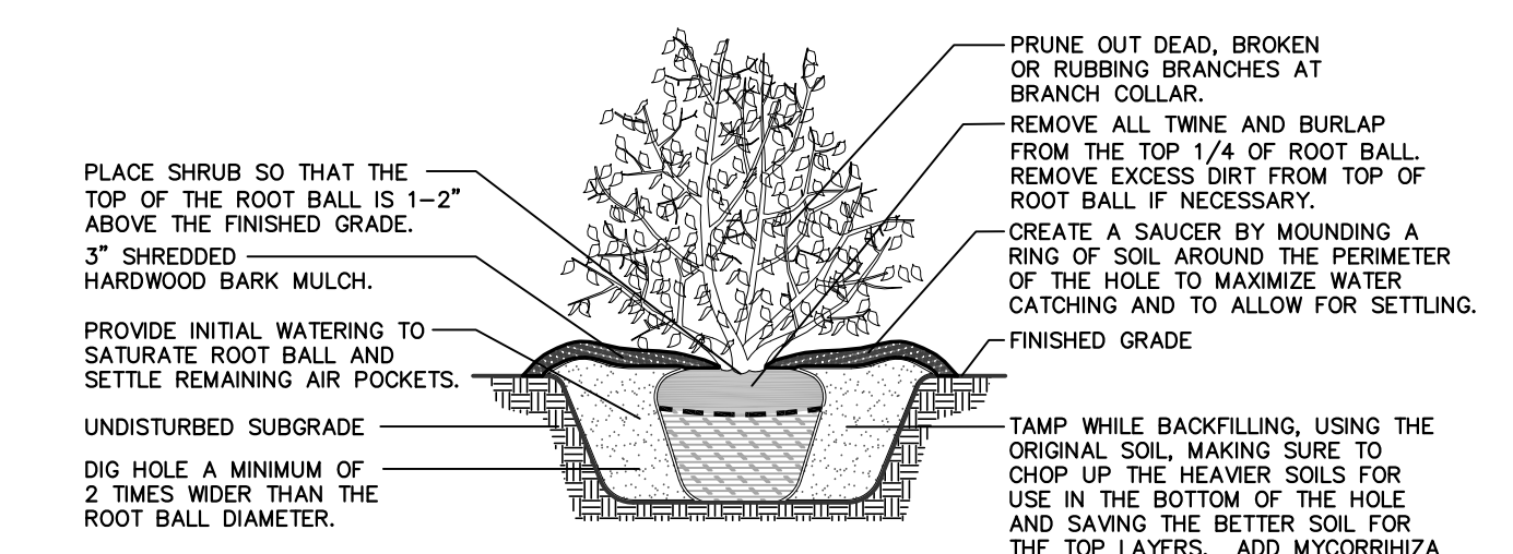
SHRUB PLANTING DETAIL NOT TO SCALE. USE ONLY ZONE HARDY PLANT MATERIAL.
